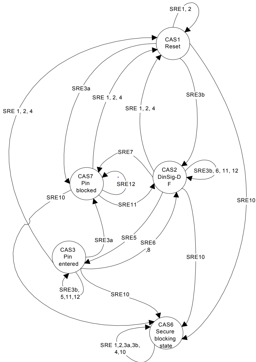
Figure 5: State transition
